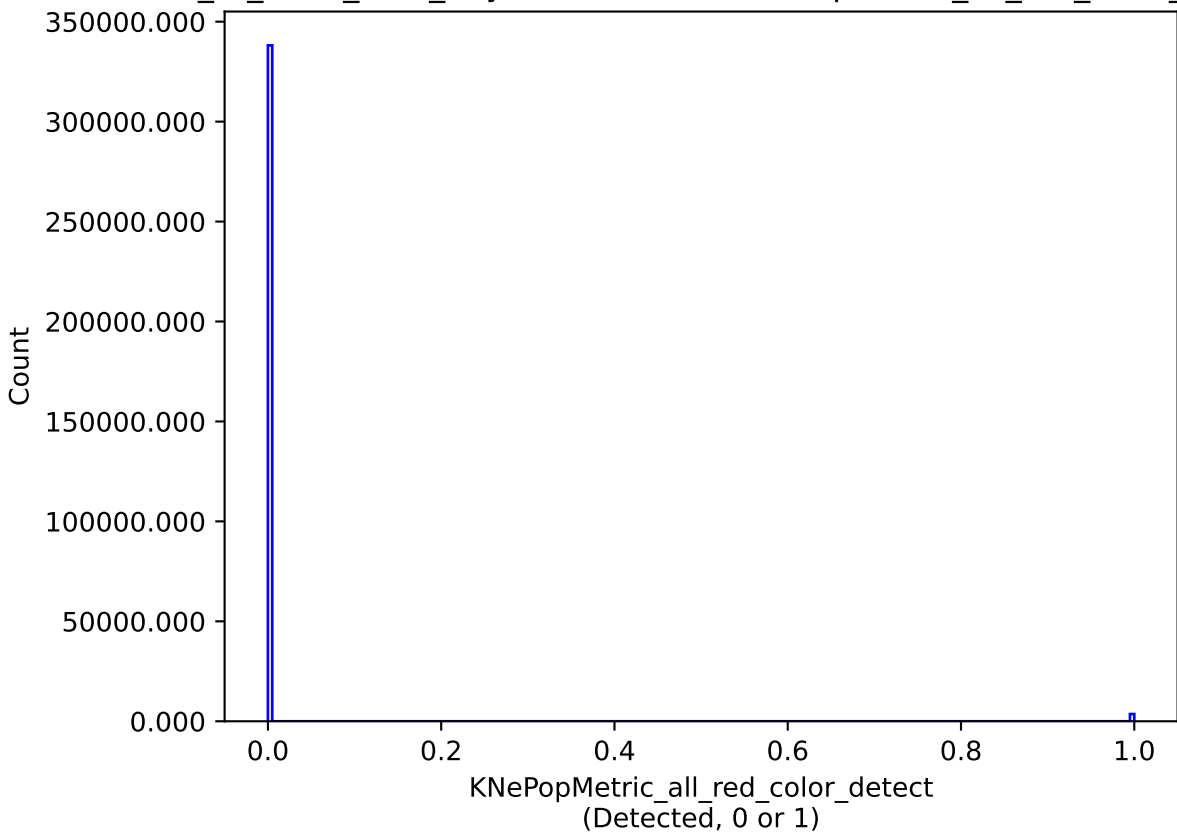
extra_ss_neo5_v3.4_10yrs all models: KNePopMetric_all_red_color_detect
