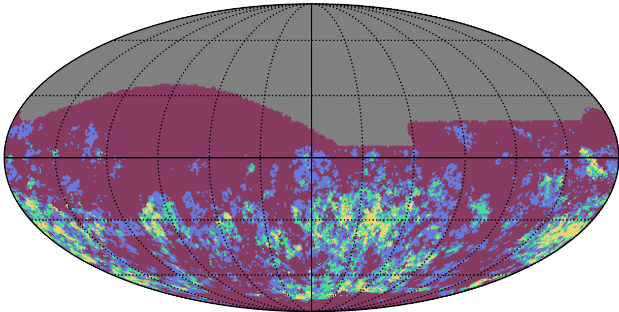
extra_ss_neo5_v3.4_10yrs z band: Gaps_7hr
