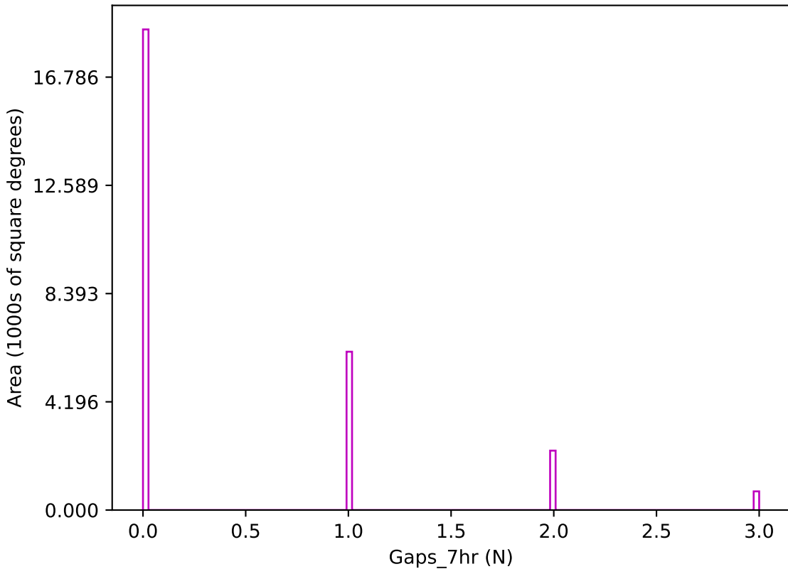
extra_ss_neo5_v3.4_10yrs z band: Gaps_7hr
