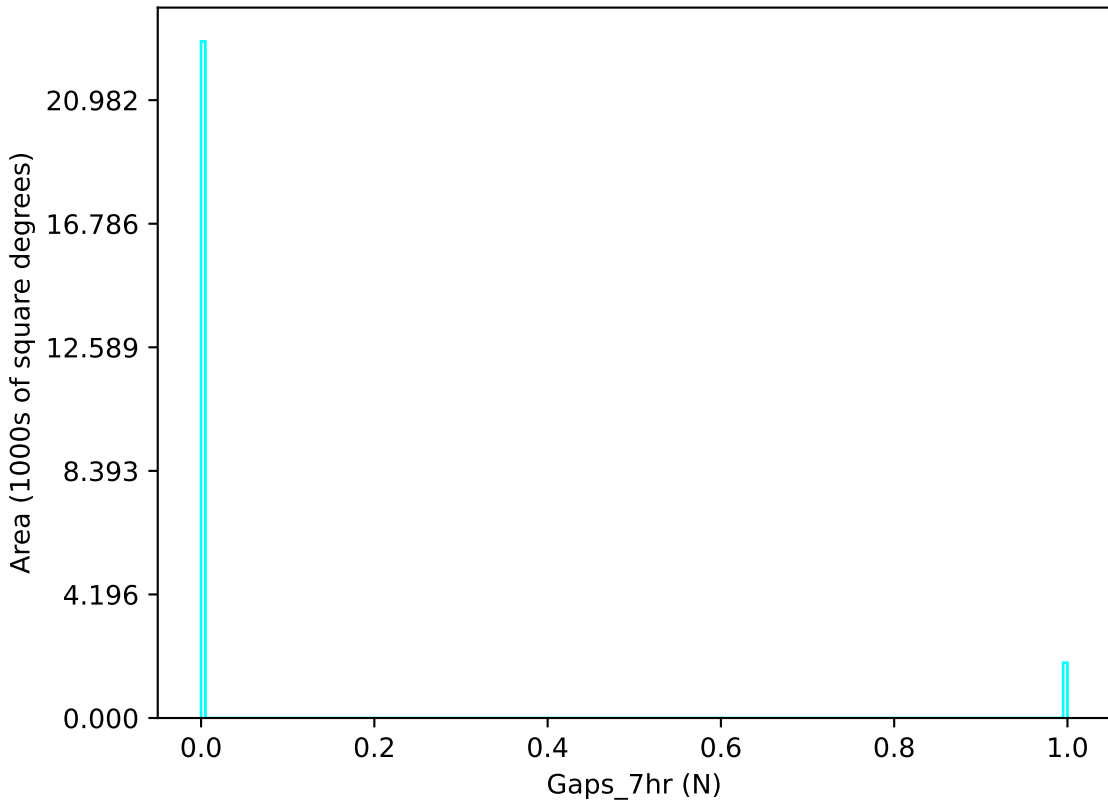
extra_ss_neo5_v3.4_10yrs u band: Gaps_7hr
