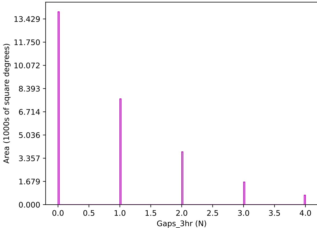
extra_ss_neo5_v3.4_10yrs z band: Gaps_3hr
