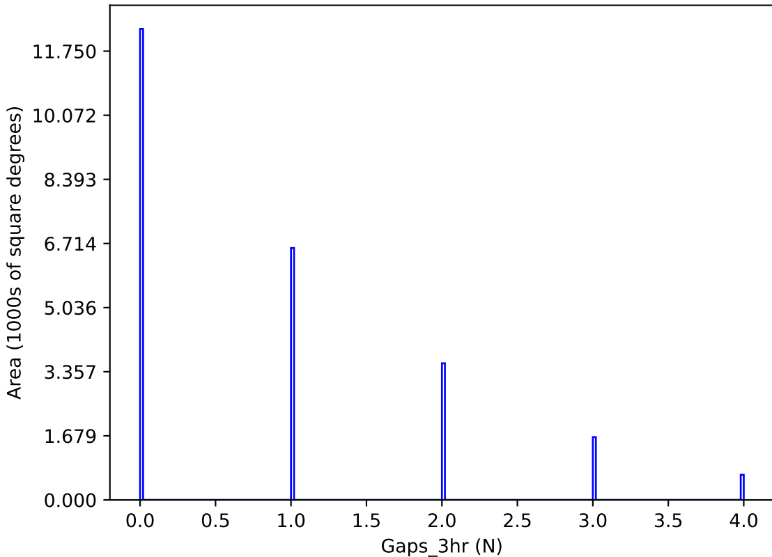
extra_ss_neo5_v3.4_10yrs y band: Gaps_3hr
