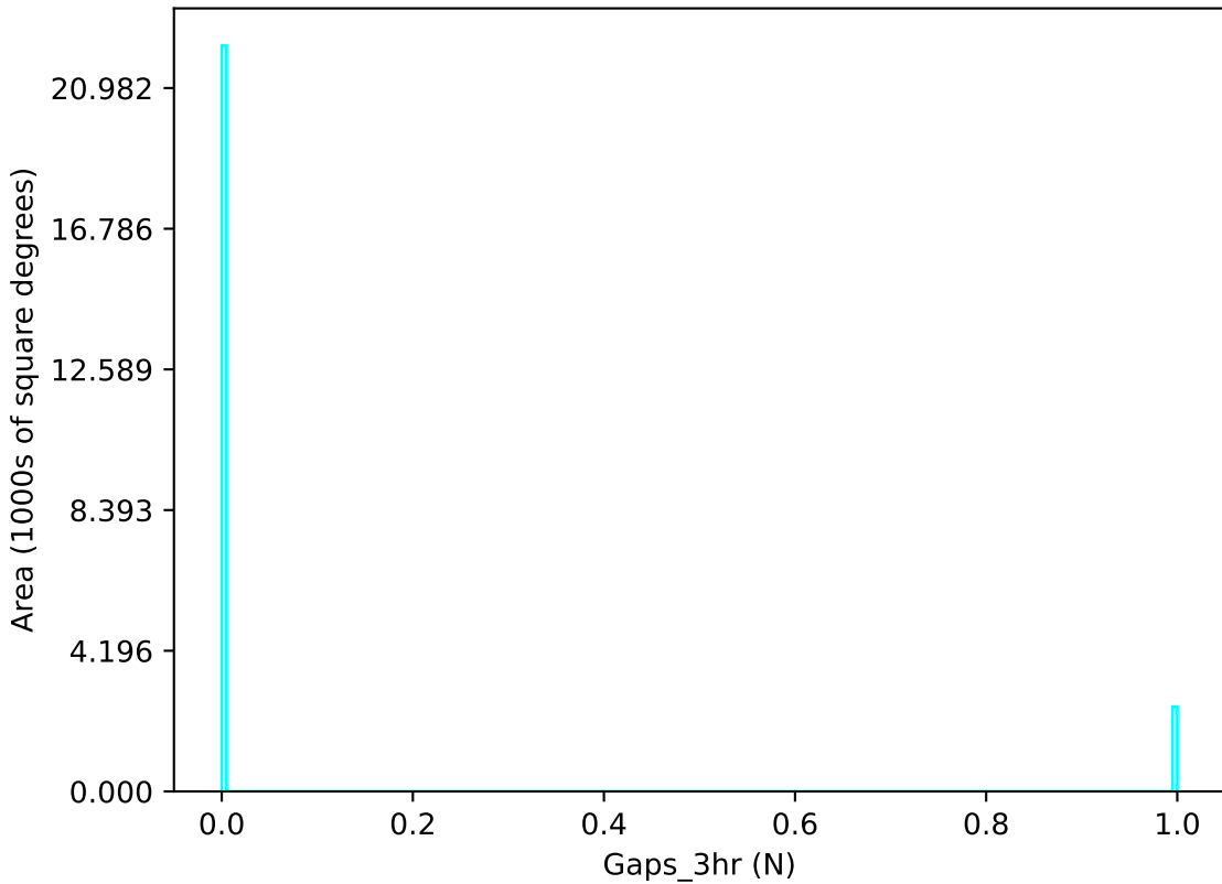
extra_ss_neo5_v3.4_10yrs u band: Gaps_3hr
