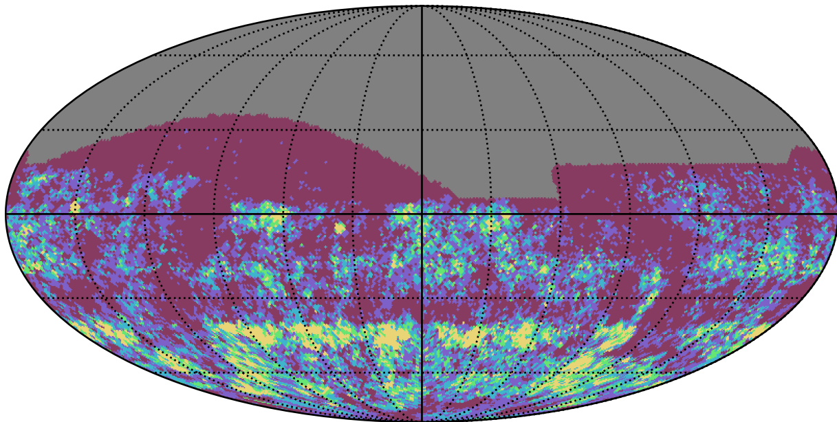
extra_ss_neo5_v3.4_10yrs r band: Gaps_3hr
