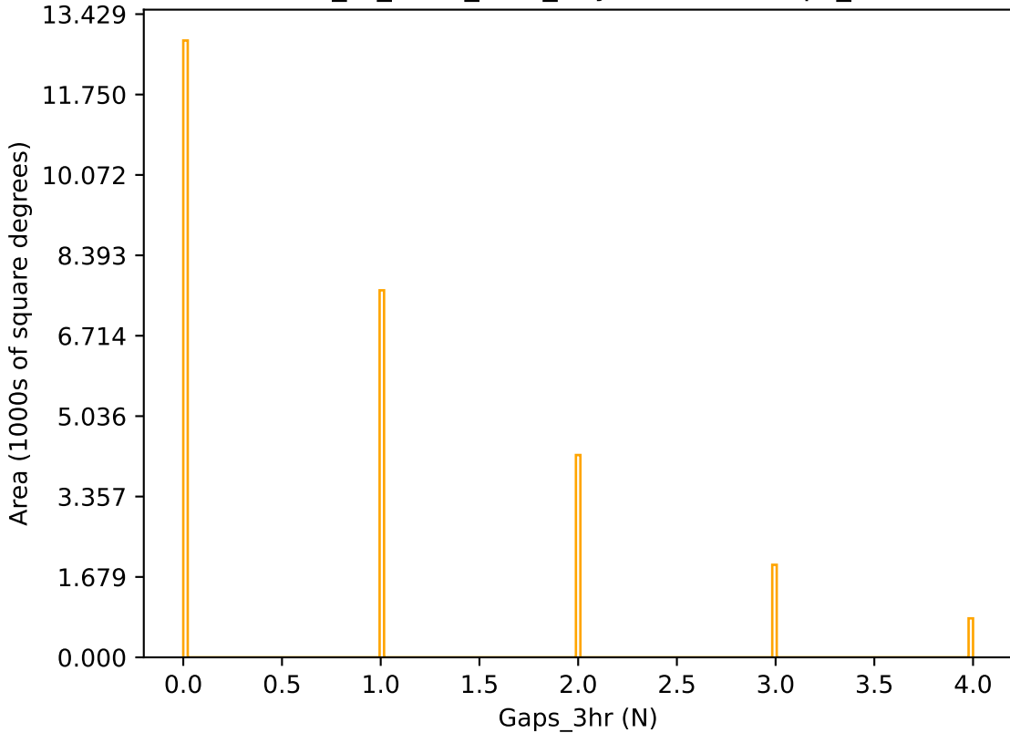
extra_ss_neo5_v3.4_10yrs r band: Gaps_3hr
