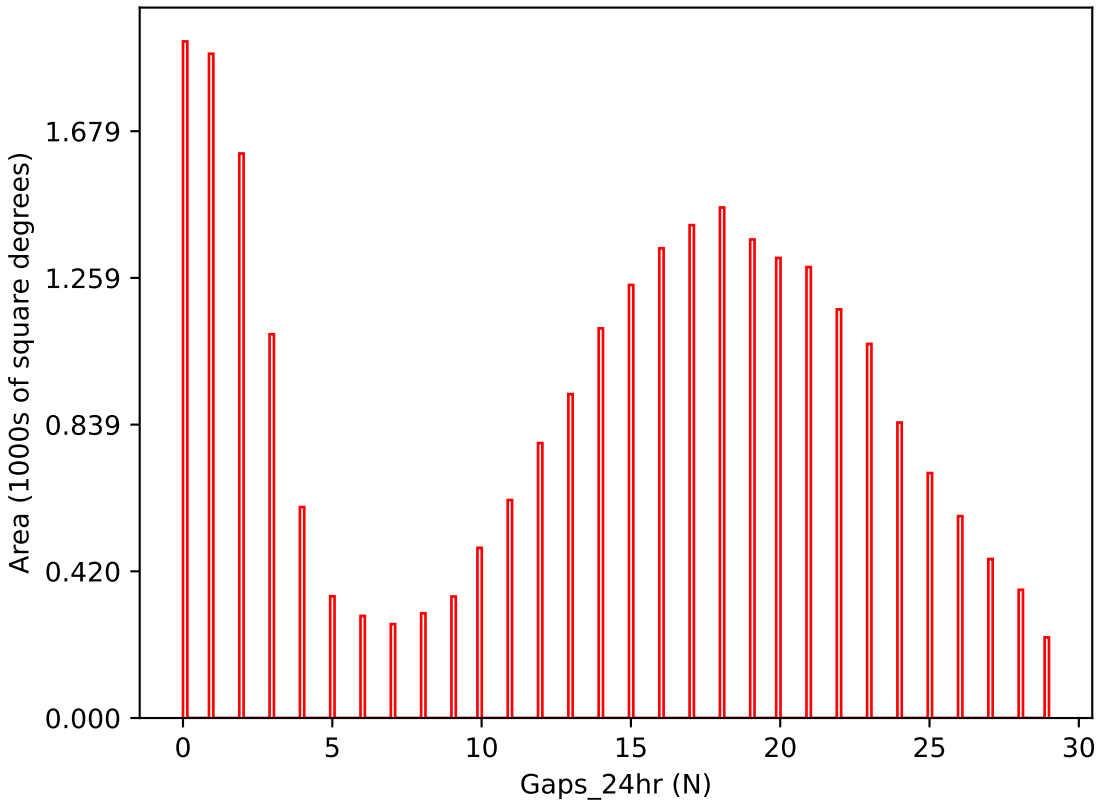
extra_ss_neo5_v3.4_10yrs i band: Gaps_24hr
