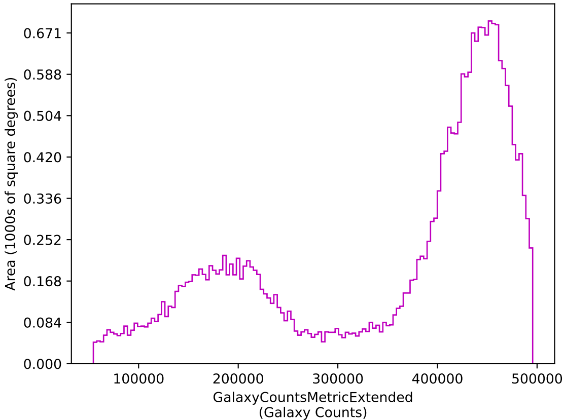
extra_ss_neo5_v3.4_10yrs z: GalaxyCountsMetricExtended
