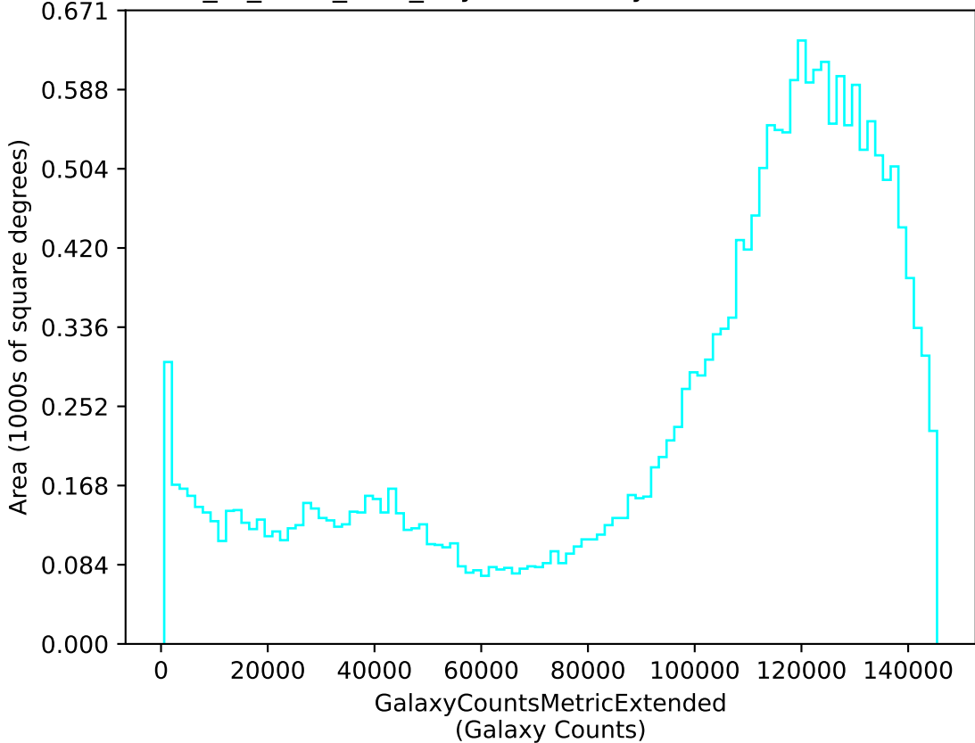
extra_ss_neo5_v3.4_10yrs u: GalaxyCountsMetricExtended
