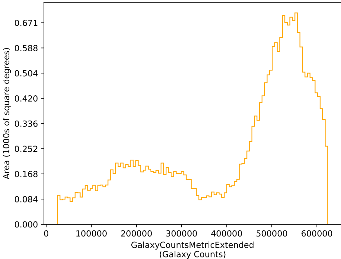
extra_ss_neo5_v3.4_10yrs r: GalaxyCountsMetricExtended
