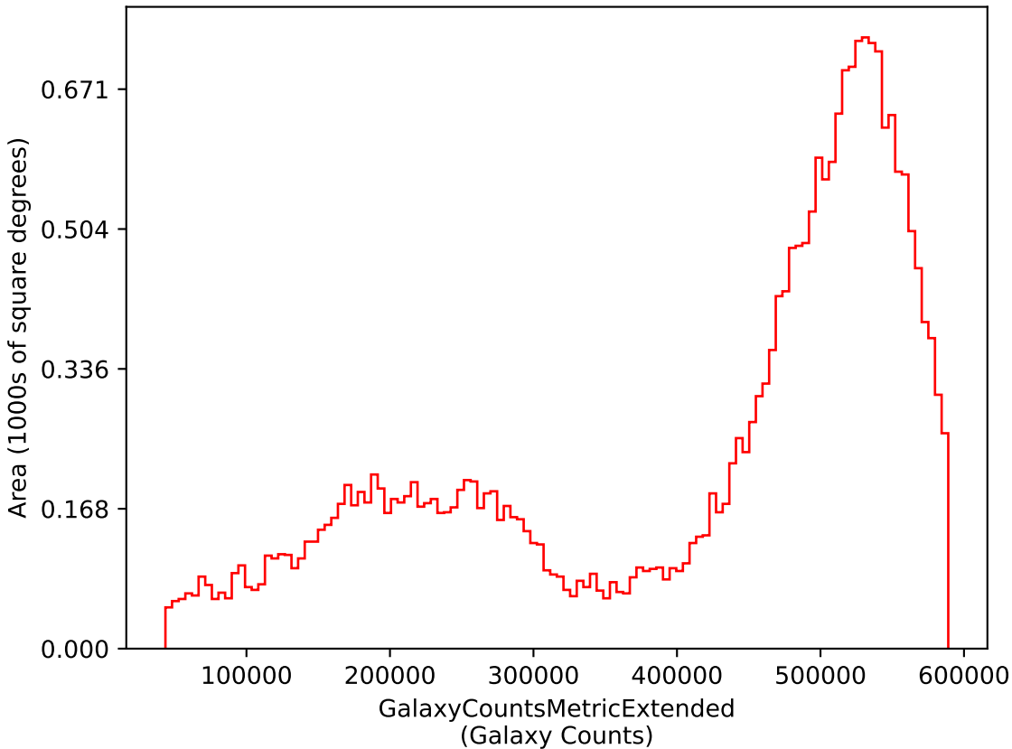
extra_ss_neo5_v3.4_10yrs i: GalaxyCountsMetricExtended
