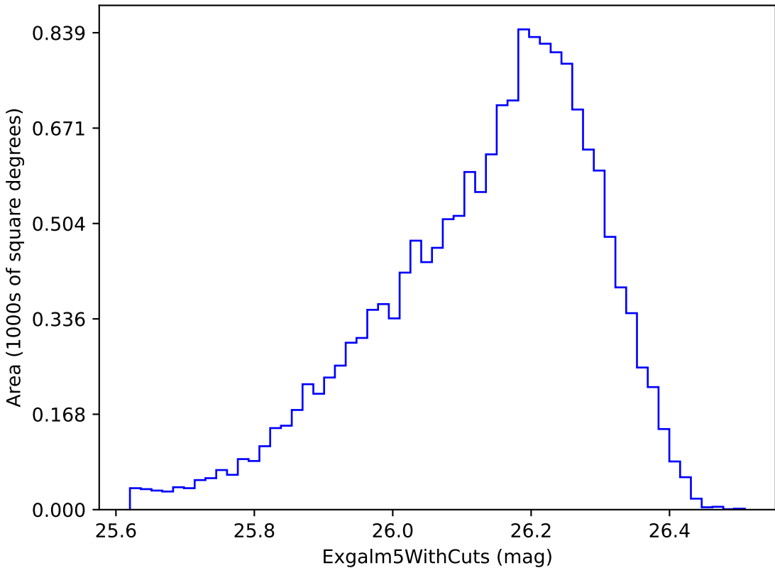
extra_ss_neo5_v3.4_10yrs i band non-DD year 6: ExgalM5WithCuts
