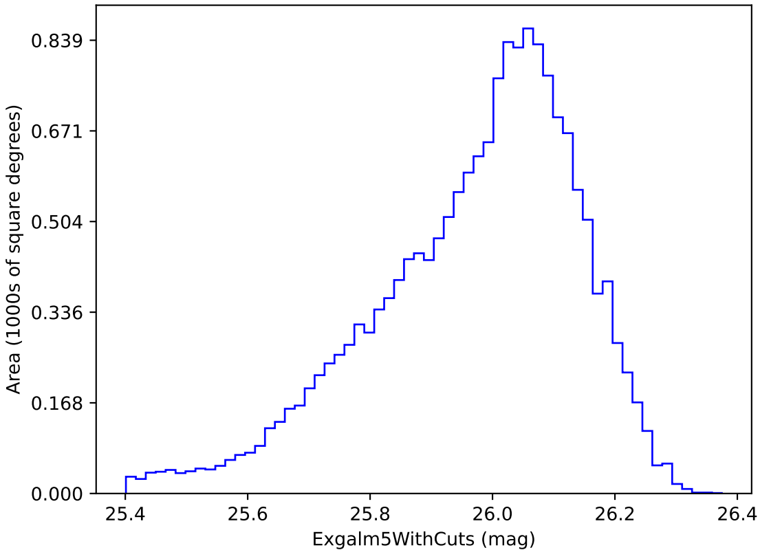
extra_ss_neo5_v3.4_10yrs i band non-DD year 4: ExgalM5WithCuts
