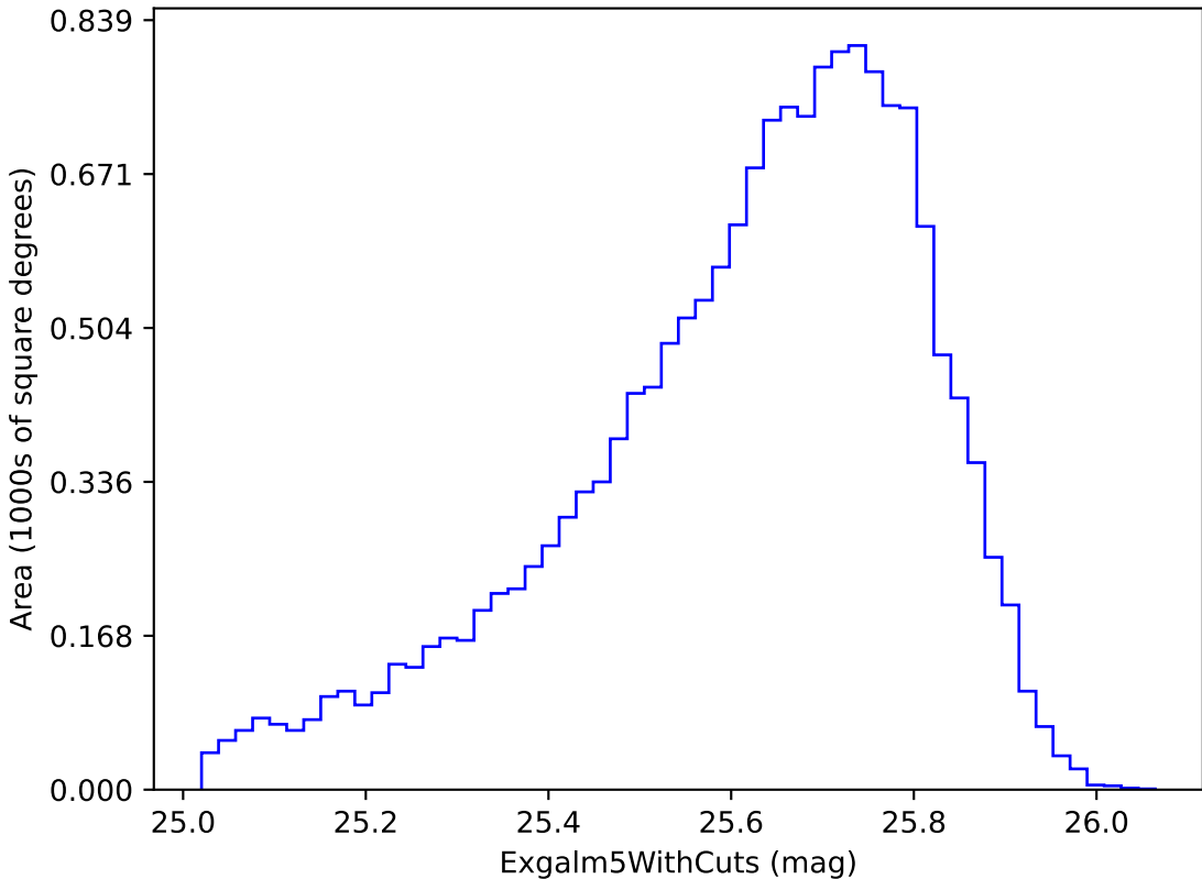
extra_ss_neo5_v3.4_10yrs i band non-DD year 2: ExgalM5WithCuts
