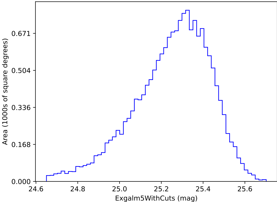
extra_ss_neo5_v3.4_10yrs i band non-DD year 1: ExgalM5WithCuts
