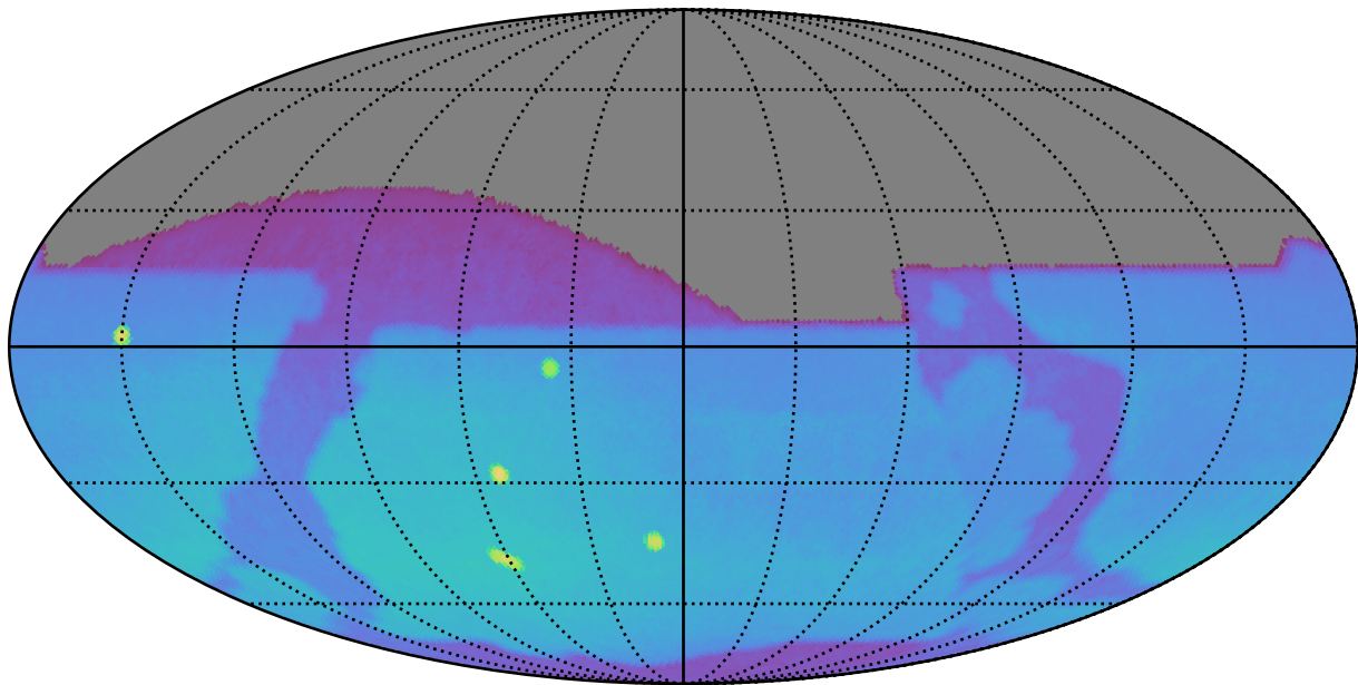
extra_ss_neo5_v3.4_10yrs : Brown Dwarf, L7
