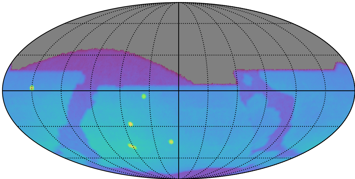
extra_ss_neo5_v3.4_10yrs : Brown Dwarf, L4
