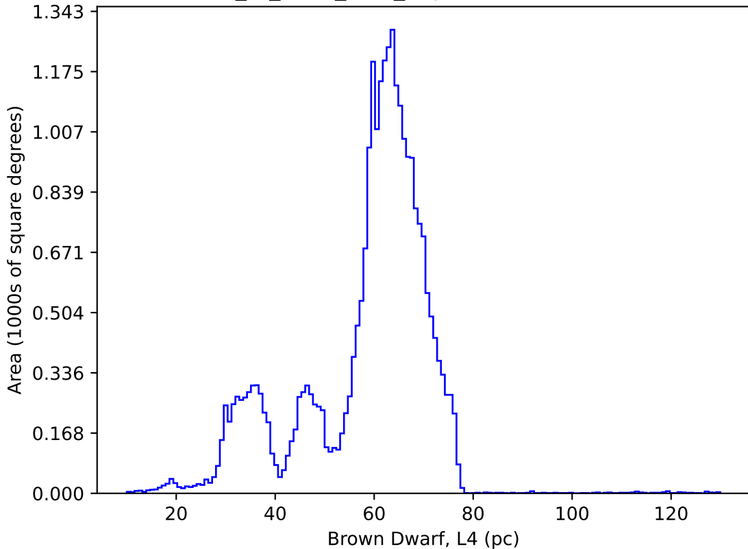
extra_ss_neo5_v3.4_10yrs : Brown Dwarf, L4
