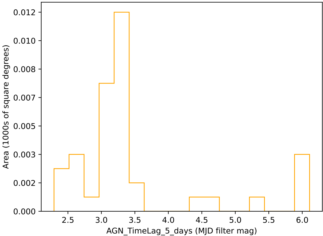
extra_ss_neo5_v3.4_10yrs r band: AGN_TimeLag_5_days
