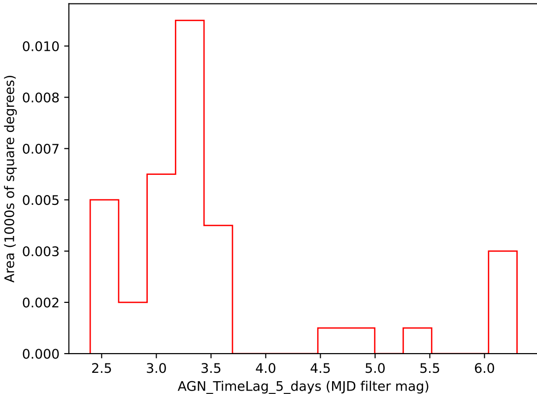
extra_ss_neo5_v3.4_10yrs i band: AGN_TimeLag_5_days
