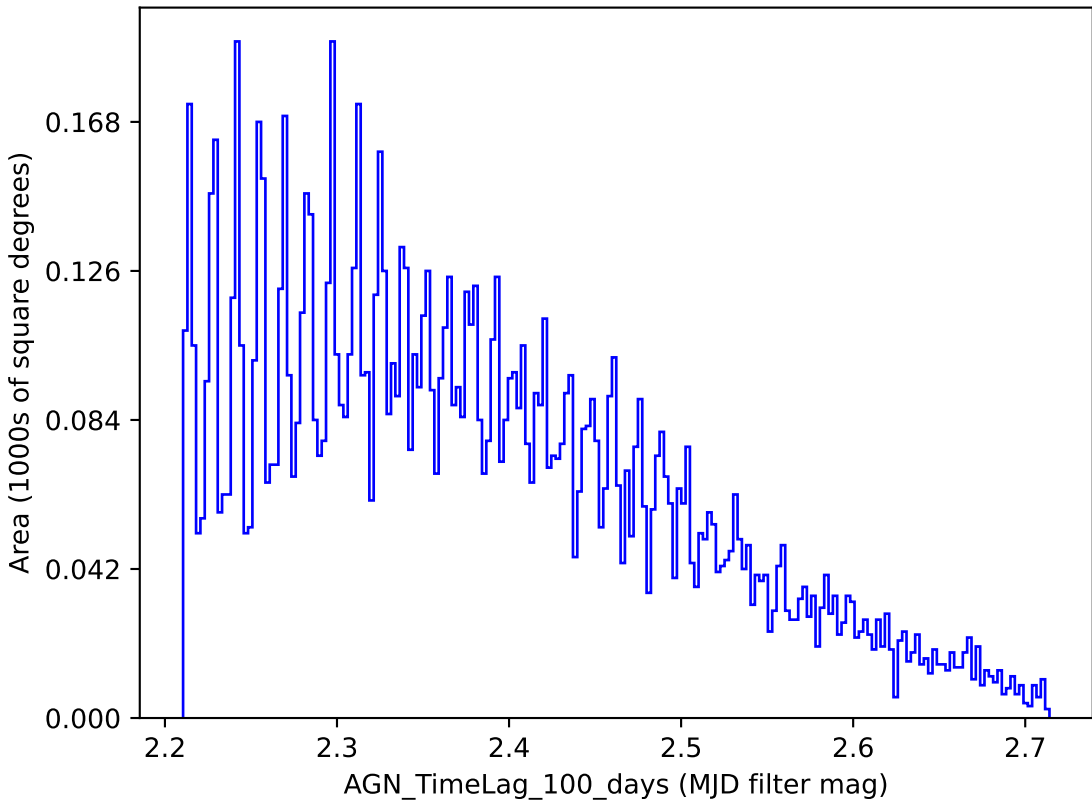
extra_ss_neo5_v3.4_10yrs y band: AGN_TimeLag_100_days
