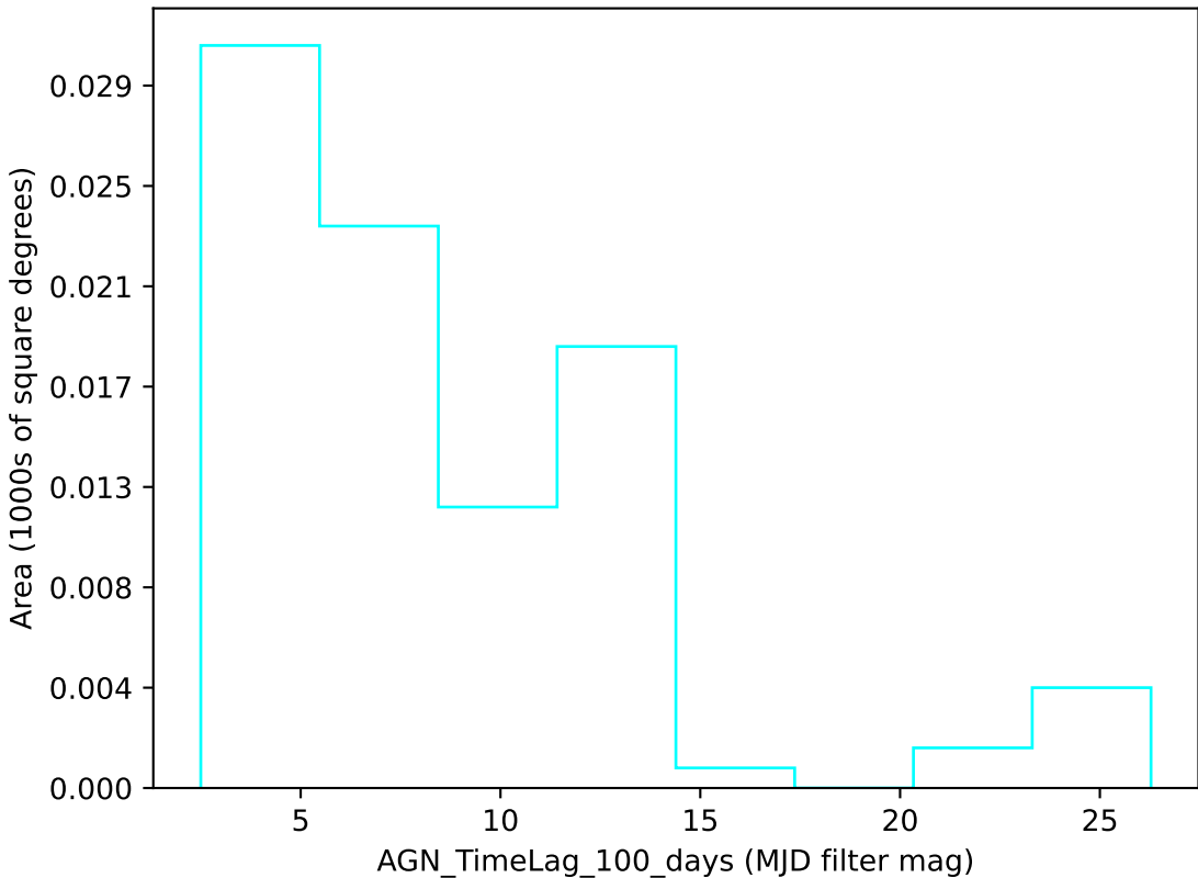
extra_ss_neo5_v3.4_10yrs u band: AGN_TimeLag_100_days
