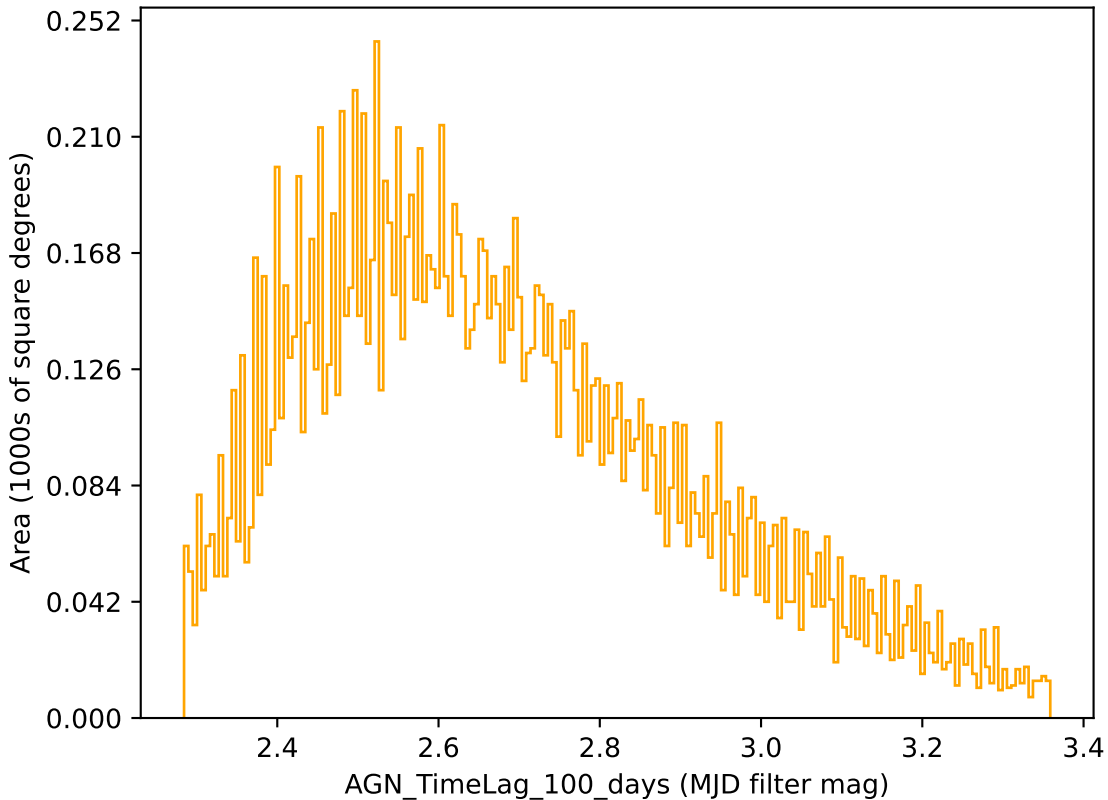
extra_ss_neo5_v3.4_10yrs r band: AGN_TimeLag_100_days
