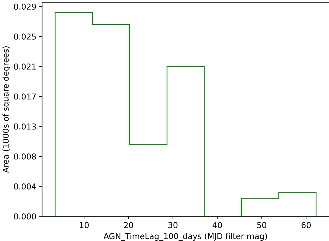
extra_ss_neo5_v3.4_10yrs g band: AGN_TimeLag_100_days
