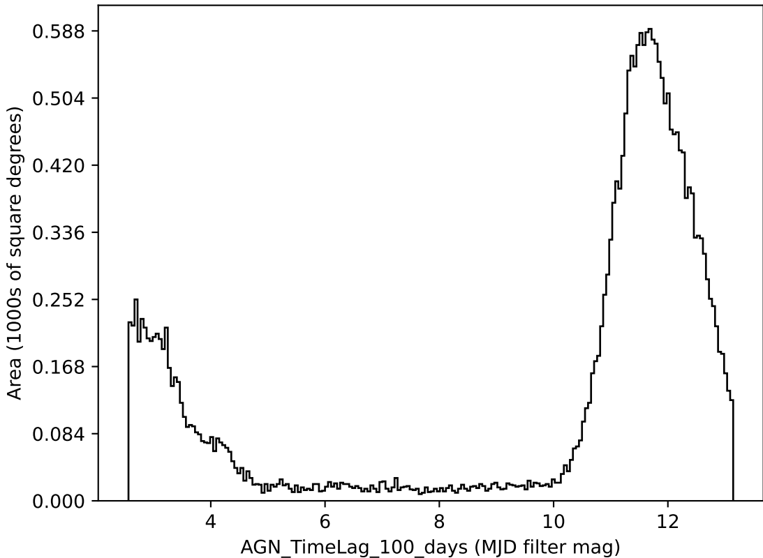
extra_ss_neo5_v3.4_10yrs all bands: AGN_TimeLag_100_days
