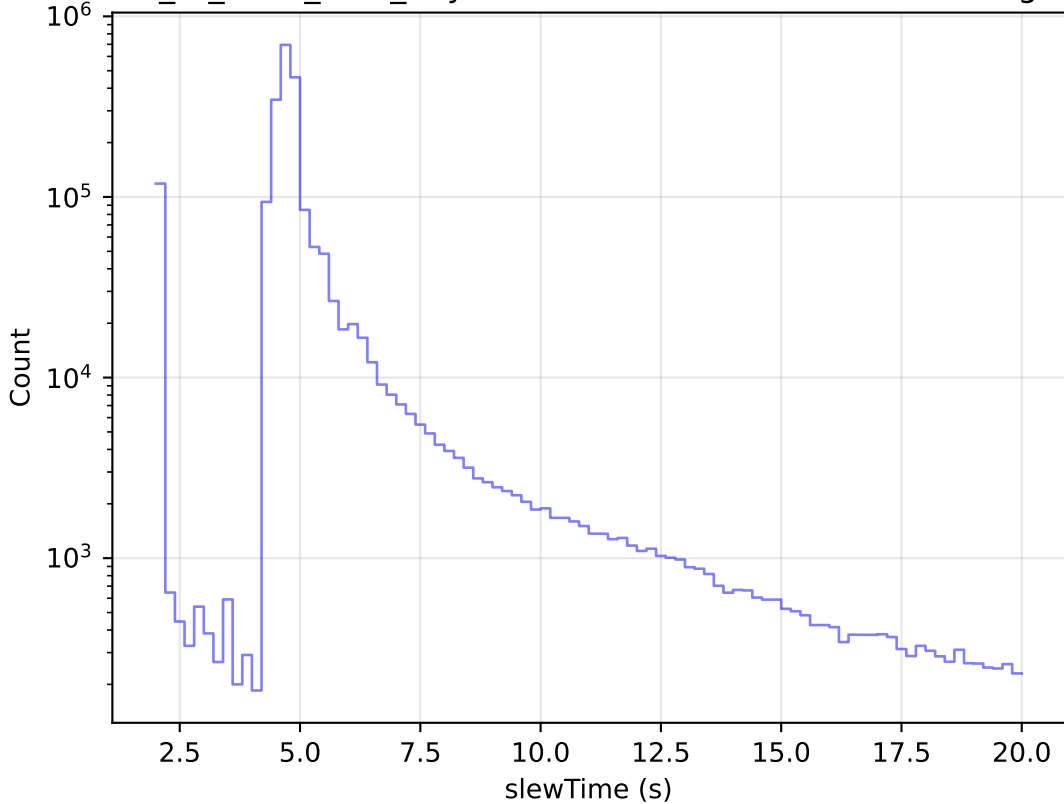
extra_ss_neo5_v3.4_10yrs All visits: Zoom Slew Time Histogram
