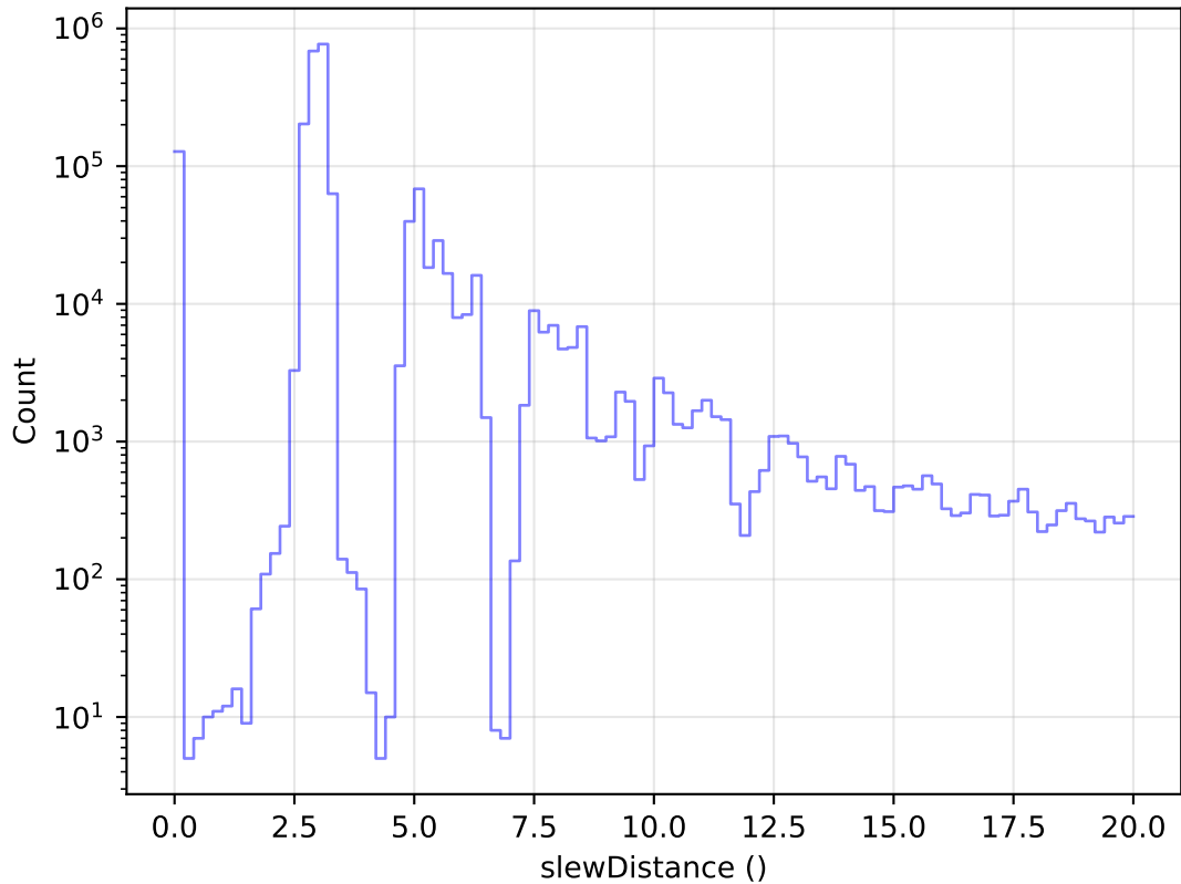
extra_ss_neo5_v3.4_10yrs All visits: Zoom Slew Distance Histogram
