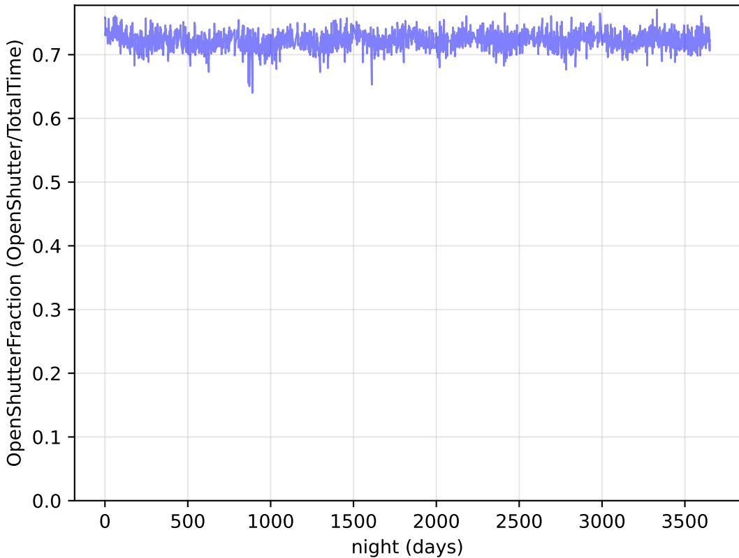
extra_ss_neo5_v3.4_10yrs : OpenShutterFraction
