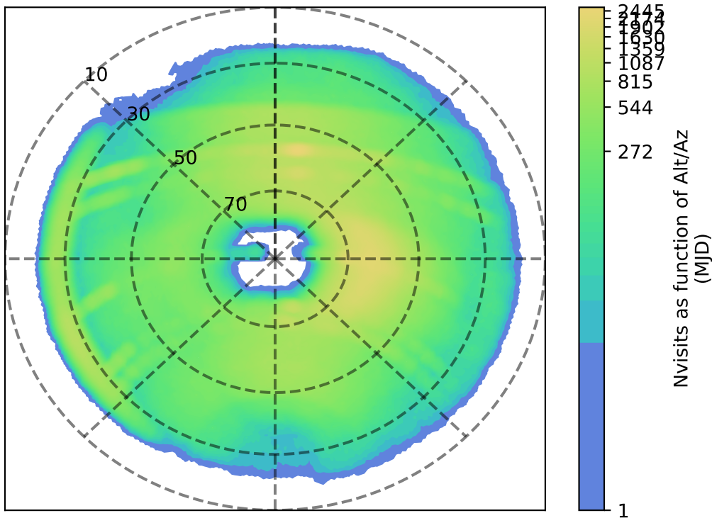
extra_ss_neo5_v3.4_10yrs r: Nvisits as function of Alt/Az
