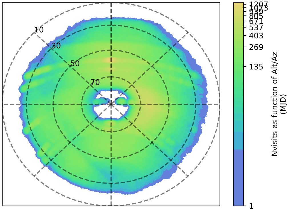
extra_ss_neo5_v3.4_10yrs g: Nvisits as function of Alt/Az
