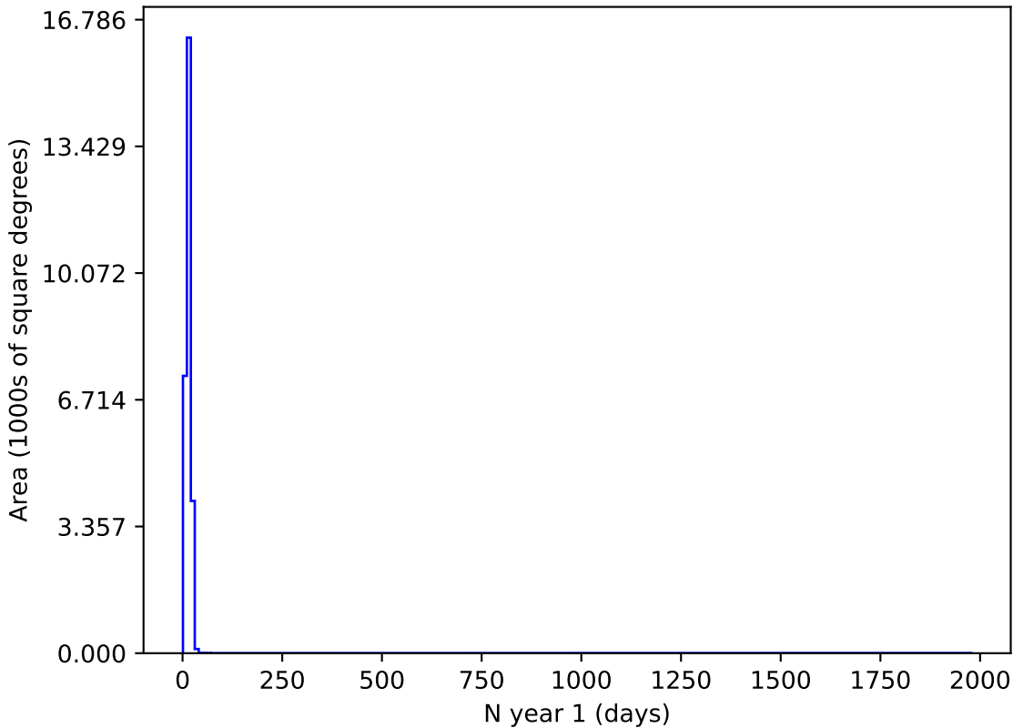
extra_ss_neo5_v3.4_10yrs z and night < 365: N year 1
