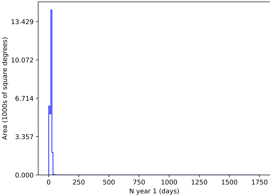
extra_ss_neo5_v3.4_10yrs i and night < 365: N year 1
