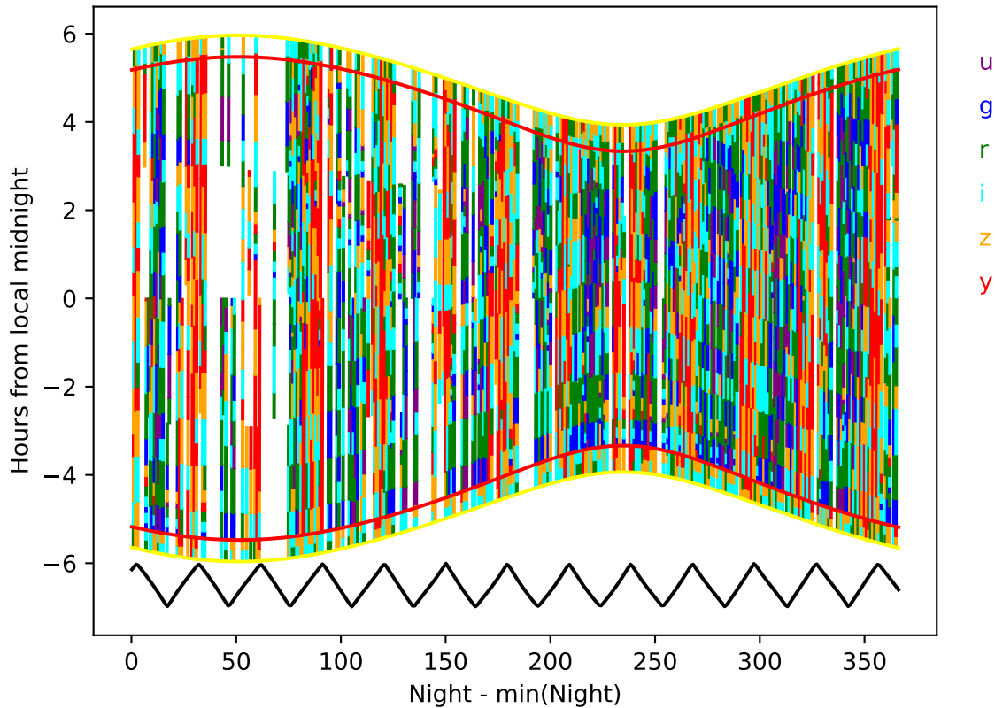
extra_ss_neo5_v3.4_10yrs year 9-10: Hourglass
