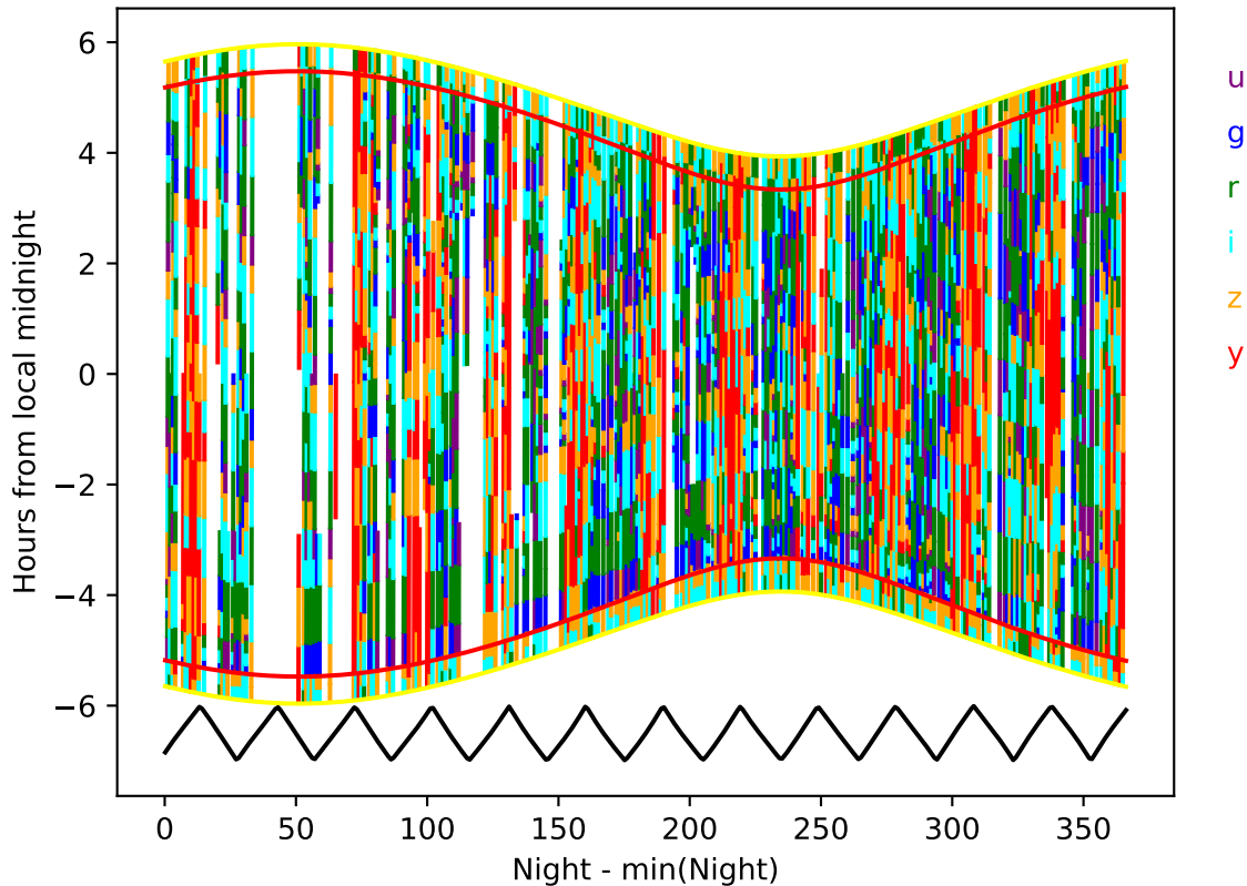
extra_ss_neo5_v3.4_10yrs year 8-9: Hourglass
