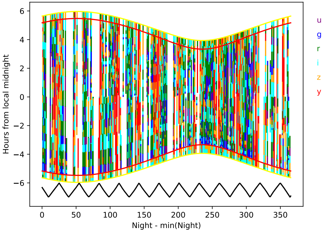
extra_ss_neo5_v3.4_10yrs year 7-8: Hourglass
