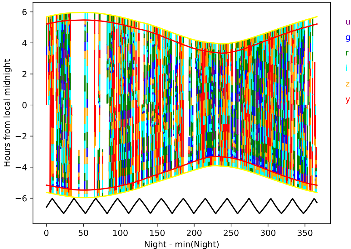
extra_ss_neo5_v3.4_10yrs year 3-4: Hourglass
