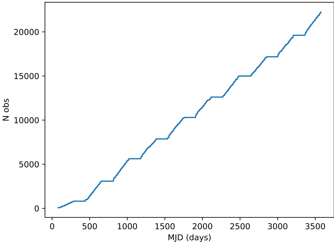
extra_ss_neo5_v3.4_10yrs note like DD:XMM_LSS%: Cumulative
