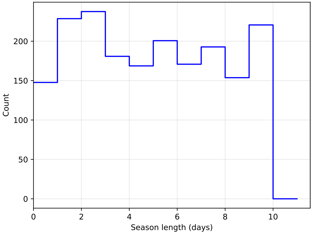
extra_ss_neo5_v3.4_10yrs DD:WFD all bands: SeasonLength
