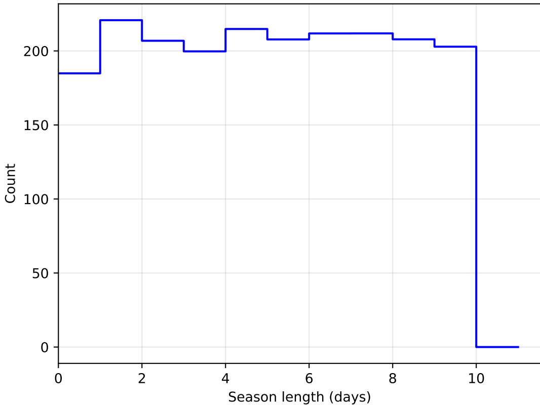
extra_ss_neo5_v3.4_10yrs DD:ELAISS1 all bands: SeasonLength
