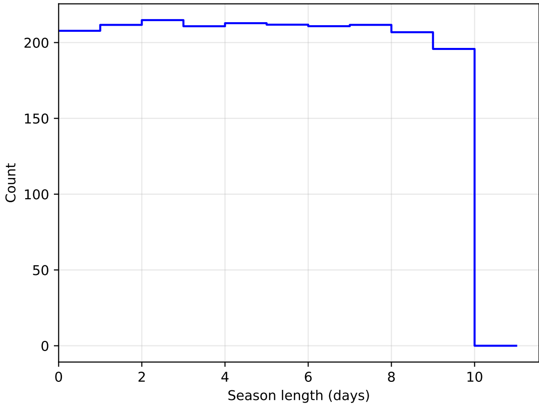
extra_ss_neo5_v3.4_10yrs DD:EDFS all bands: SeasonLength
