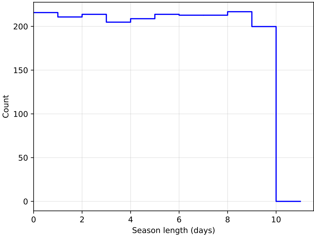
extra_ss_neo5_v3.4_10yrs DD:ECDFS all bands: SeasonLength
