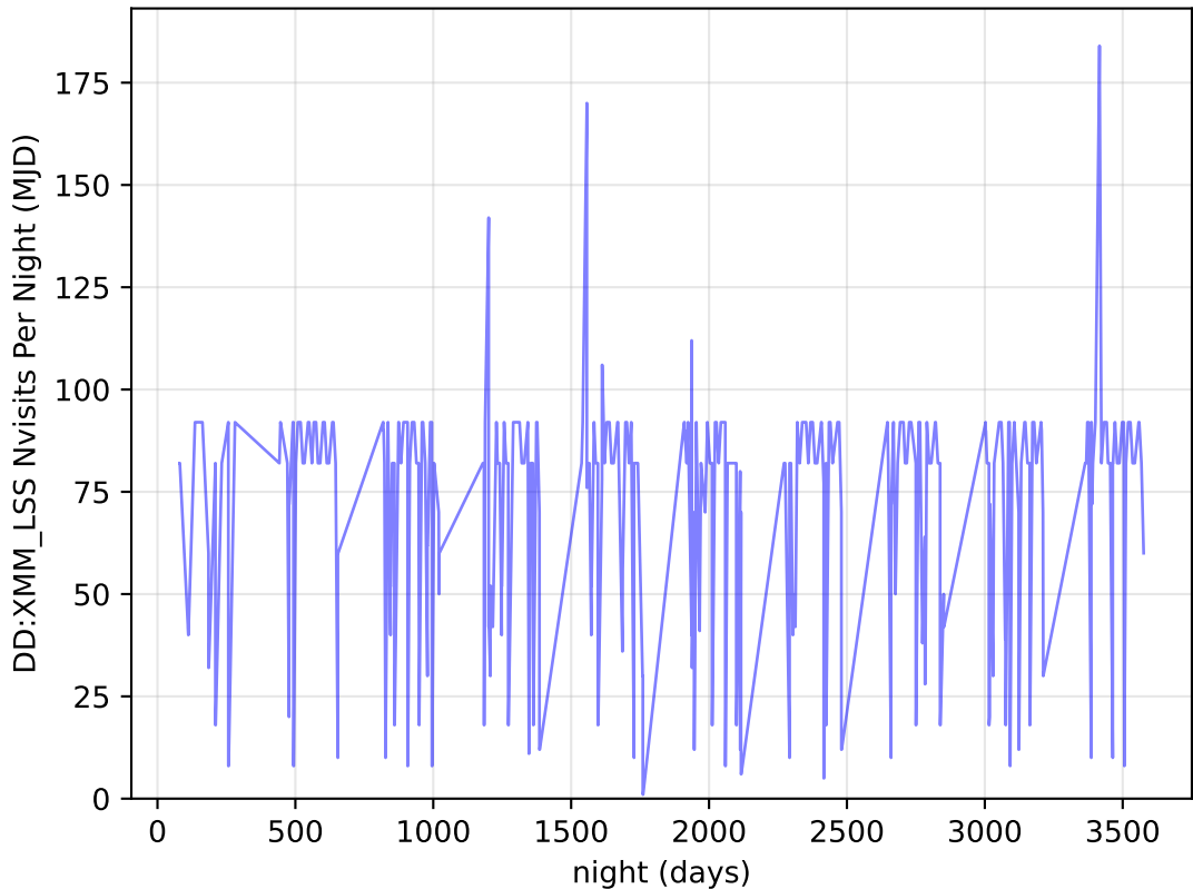
extra_ss_neo5_v3.4_10yrs all bands: DD:XMM_LSS Nvisits Per Night
