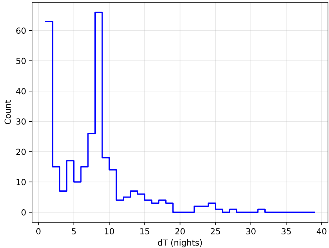
extra_ss_neo5_v3.4_10yrs all bands: DD:XMM_LSS Delta Nights Histogram
