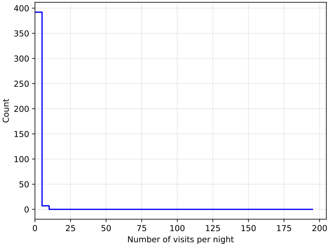
extra_ss_neo5_v3.4_10yrs all bands: DD:WFD NVisitsPerNight
