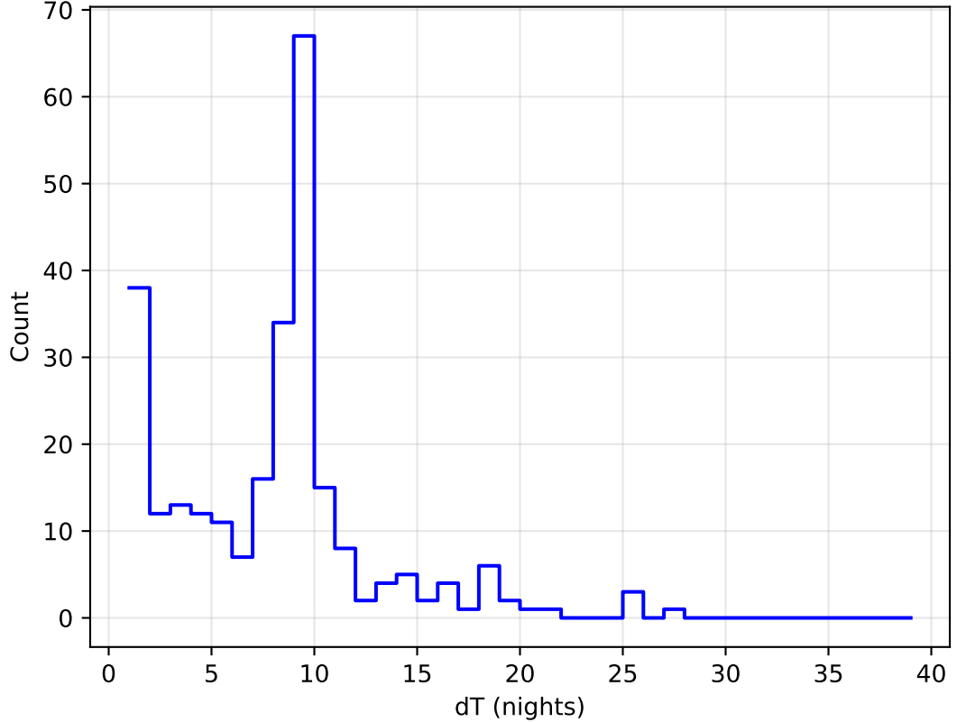
extra_ss_neo5_v3.4_10yrs all bands: DD:ELAISS1 Delta Nights Histogram
