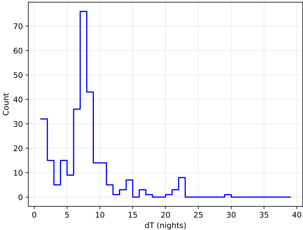
extra_ss_neo5_v3.4_10yrs all bands: DD:EDFS Delta Nights Histogram
