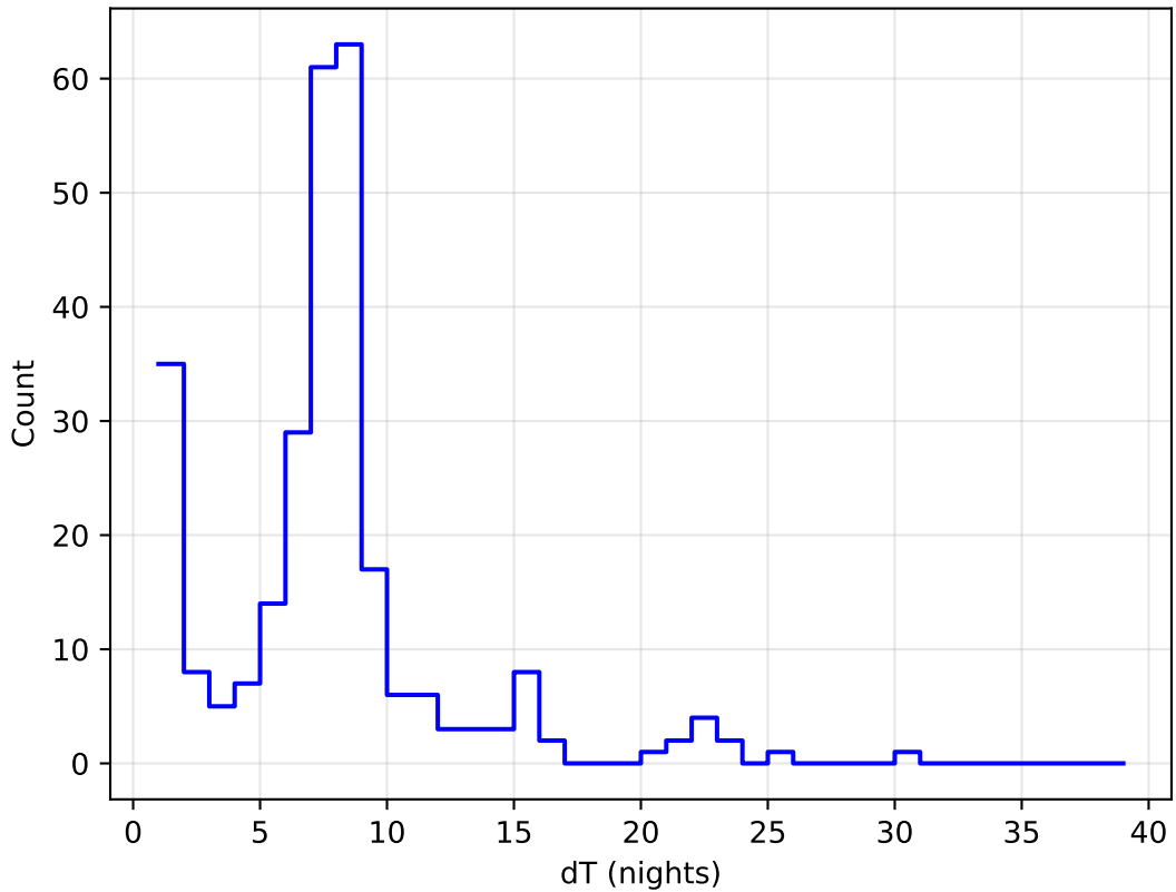
extra_ss_neo5_v3.4_10yrs all bands: DD:ECDFS Delta Nights Histogram
